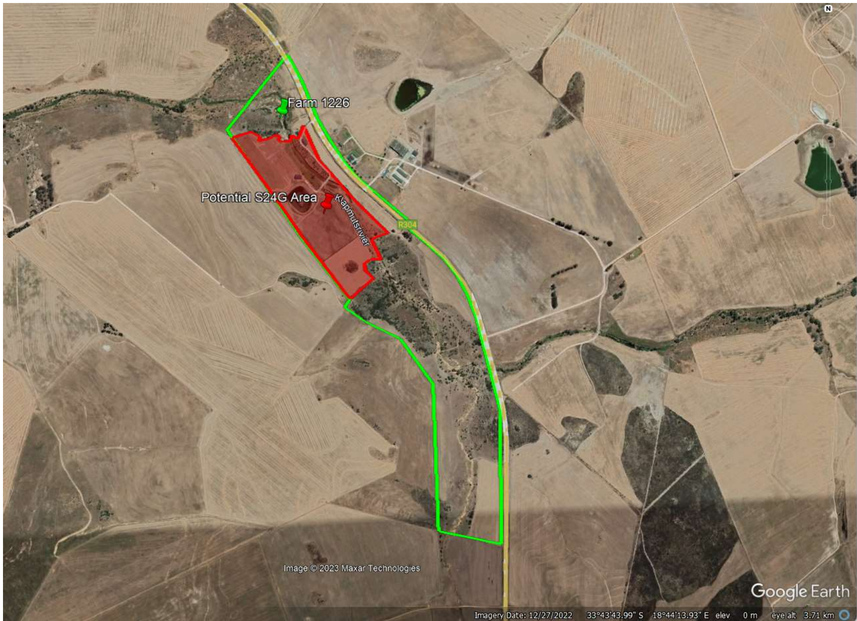
Satellite image indicating area (indicated in red) on Olienhouts Kloof Farm 1226 (outlined in green), where alleged unauthorised activities in terms of the National Environmental Management Act, No. 107 of 1998, as amended (NEMA), have commenced or are continuing which require a S24G rectification application. Olienhouts Kloof Farm 1226 is located just off the R304, Durbanville, City of Cape Town Municipality, Western Cape Province.
